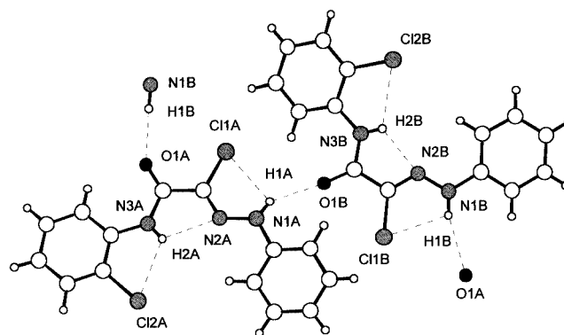
Figure 3. Structures of two independent molecules in the crystal of compound 1d , showing intra- and intermolecular hydrogen bonding (dashed lines)
