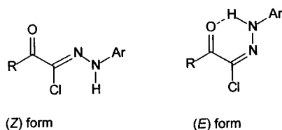
Scheme 4. Isomeric forms of \alpha -carbonyl-substituted hydrazonoyl chlorides
