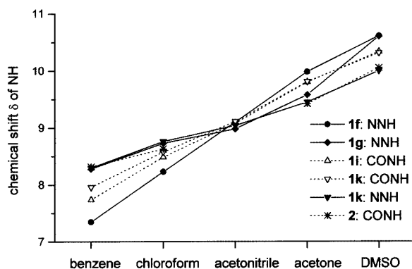
Figure 5. Solvent dependence of the chemical shifts ( \delta ) of the anilide (CONH, open symbols) and the hydrazone (NNH, closed symbols) protons
