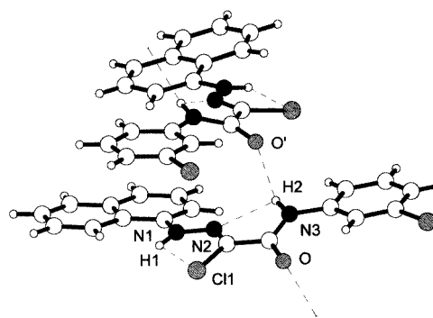
Figure 4. Structure of two molecules in the crystal of compound 1k , showing intra- and intermolecular hydrogen bonding (dashed lines)
