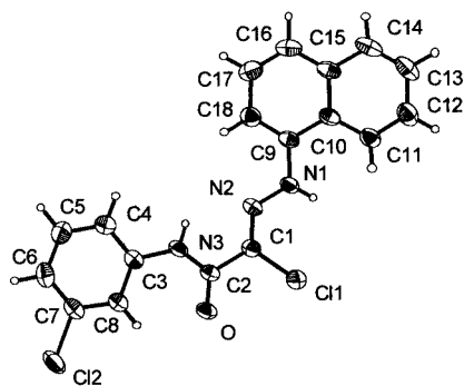
Figure 2. Molecular structure of 1k with atom-numbering scheme (displacement ellipsoids with 50% probability)
