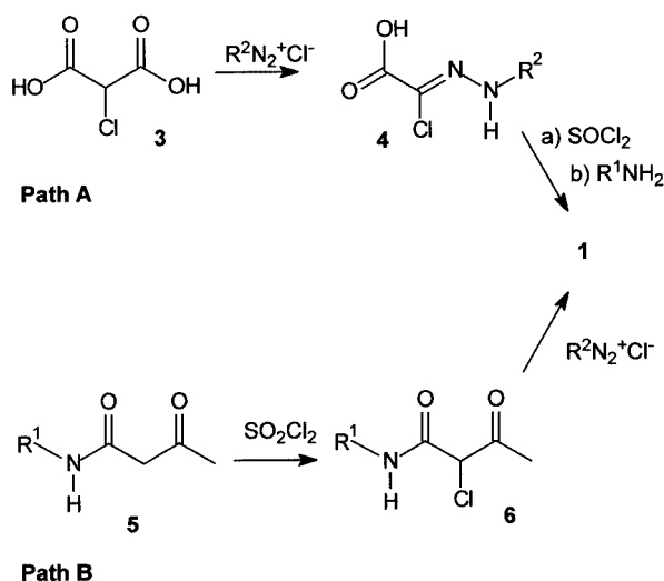
Scheme 1. Routes to oxamo- N -arylhydrazonoyl chlorides
