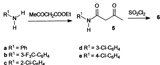
Scheme 2. Synthesis of 2-chloro-3-oxobutanamides 6
