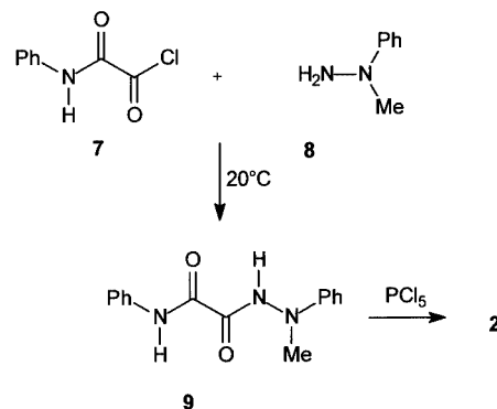
Scheme 3. Synthesis of oxanilo- N -methyl- N -phenylhydrazonoyl chloride ( 2 )
