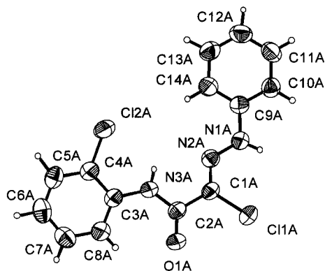
Figure 1. Molecular structure and atom-numbering scheme of one of the two independent molecules of 1d (displacement ellipsoids with 50% probability)
