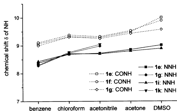
Figure 6. Solvent dependence of the chemical shifts ( \delta ) of the anilide (CONH, open symbols) and the hydrazone (NNH, closed symbols) protons
